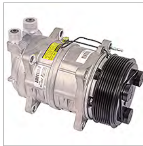
03-00870 (MANEX 03-00870) COMPRESSOR TM-16HD VOR CAST 123MM PV6 12V
