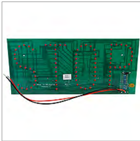
00067819 (SMI® 19-200) BOARD,LED,STOP ARM,SCHOOL BUS
