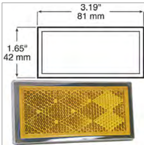
00026511 REFLECTOR,AMBER
