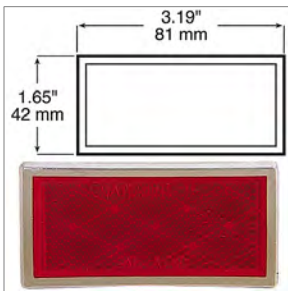
00026512 REFLECTOR,RED
