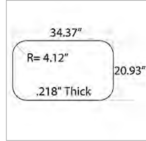
01163195 GLASS,RED,UPPER,DARK TINT LAMINATED
