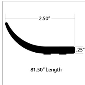
01637545 RUBBER, NOSING, EXIT PJK DOOR, FRONT
