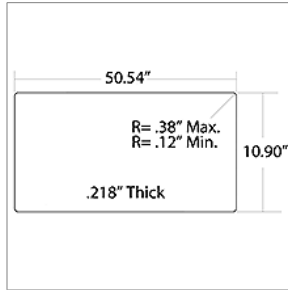
01781343 GLASS, LWR, O/O ENT DR, LAM CLR, 27.50 CV
