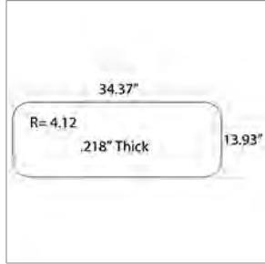
01110089 GLASS,RED,LOWER,TEMPERED
