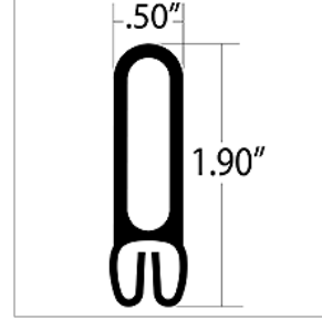
00063055 SEAL,DOOR,.50 BULB X 1.90 FLG MT,UNI-GRIP
