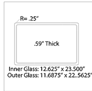
10032316 GLASS ASSY,STORM,O/O ENT DR,UPPER,TINT,A3
