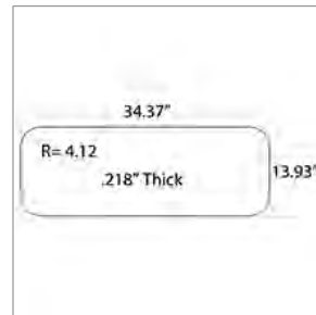
01858653 GLASS,RED,LOWER,DARK TINT,TEMPERED
