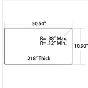
01780535 GLASS, LWR, O/O ENT DR, LAM 70 LT GRN 27.50 CV
