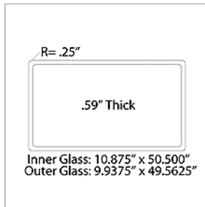
10032309 GLASS ASSY,STORM,O/O DR,LWR,27.50,LAM
