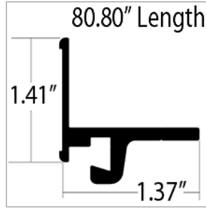
01988435 HINGE, TOP SECTION, ENGINE COMP DOOR
