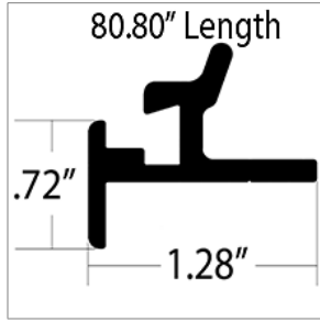
01842152 HINGE,BOTTOM SECTION,ENGINE CMPT DOOR
