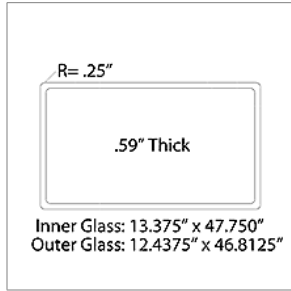
10032324 GLASS ASSY,STORM,O/O ENT DR,LWR,TINT,T3
