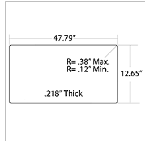
01781301 GLASS, LWR, O/O ENT DR, LAM 70 LT GRN, 24.75 TC
