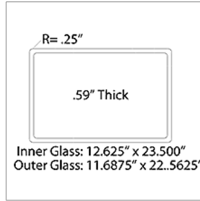
10032315 GLASS ASSY,STORM,O/O ENT DR,UPPER,A3
