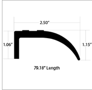
00315937 NOSING,RUBBER,ENT DOOR,O/O
