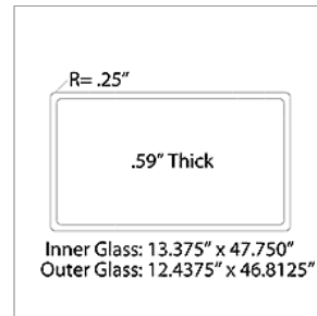
10032323 GLASS ASSY,STORM,O/O ENT DR,LWR,T3
