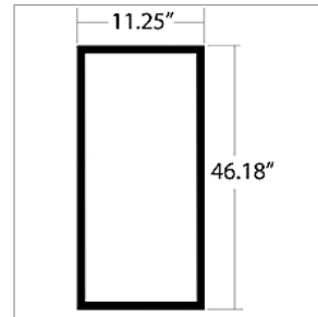
01547595 RUBBER,GLAZING,ENT DOOR LOWER CV
