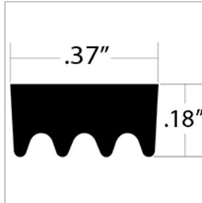
01056928 SEAL,RIB SPONGE,3/16 X 3/8 X 77.875
