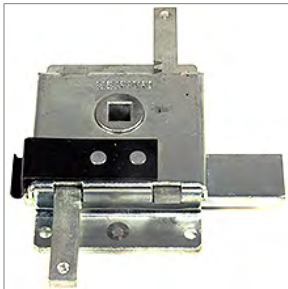
10003360 LOCK ASSY,3-PT,EMERGENCY DOOR,EBERHARD MFG, D3FE
