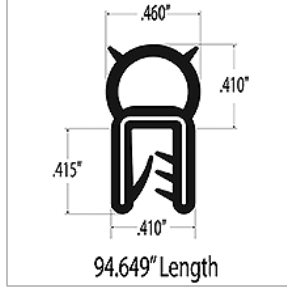
10020905 SEAL,BULB,CLIP-ON,ELECTRICAL ACCESS DOOR
