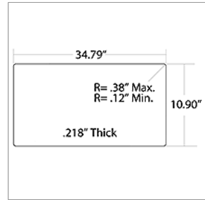
00012778 GLASS, O/O ENTRANCE DR, LAM 70% LT GREEN, B1VC
