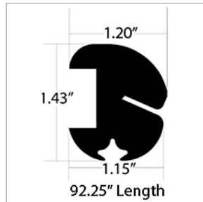
01456490 GLAZING, RUBBER, ENT DOOR, LOWER, STORM GLASS
