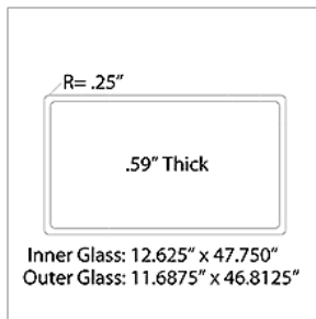
10032318 GLASS ASSY,STORM,O/O ENT DR,LWR,24.75,TINT,A3
