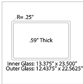
10032311 GLASS ASSY,STORM,O/O ENT DR,UPPER,T3
