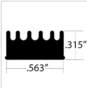
04763284 SEAL,RBR,EPDM,RIBBED,.315X.563,ADH BACK
