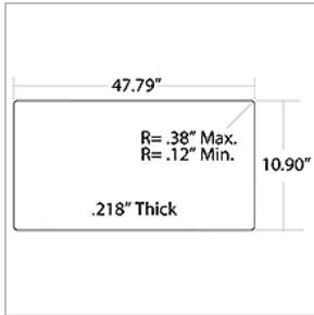
01773175 GLASS, LOWER, O/O ENT DR TEMP CLR 24.75 S CV
