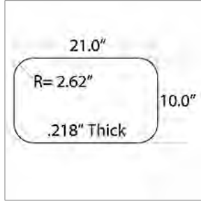
00258350 GLASS, DOOR, ENTRANCE, UPPER, TEMPERED
