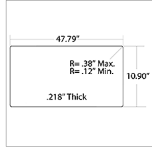
01773183 GLASS, LOWER, O/O ENT DR LAM 70 LTGRN 24.75CV
