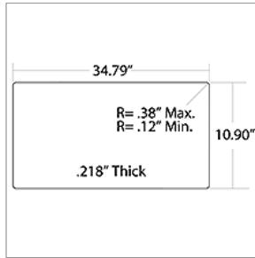
00012779 GLASS, O/O ENTRANCE DOOR, TEMPERED CLR, B1VC
