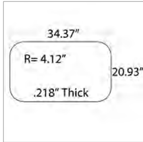
01858661 GLASS,RED,UPPER,DARK TINT TEMPERED
