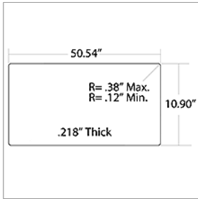
01781350 GLASS, LWR, O/O ENT DR, TEMP CLR, 27.50 CV
