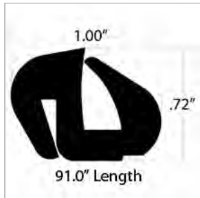
00347849 GLAZING, RUBBER, ENT DOOR, LOWER
