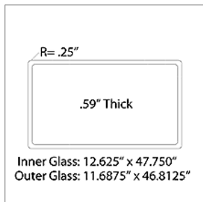
10032317 GLASS ASSY,STORM,O/O ENT DR,LWR,24.75,A3
