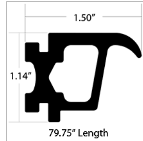
01975689 RUBBER,DOOR NOSING,O/O,V2,24.75 STEP
