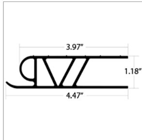
01599315 RUBBER,DOOR NOSING,FLUSH JACKKNIFE DR TC
