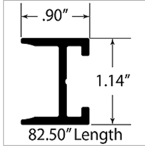
01768118 RETAINER,O/O DR NOSING FOR 27.50 STEP,82.50
