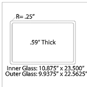
10032320 GLASS ASSY,STORM,O/O ENT DR,UPPER,TINT,CV
