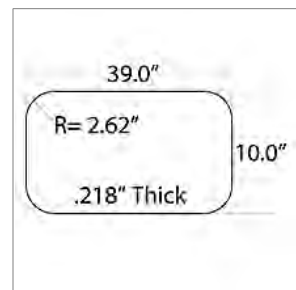
00347617 GLASS,DOOR,ENTRANCE,LOWER,CLEAR LAMINATED
