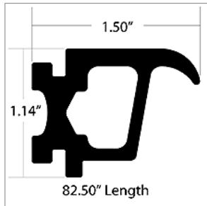
01975697 RUBBER,DOOR NOSING,O/O,V2,27.50 STEP
