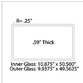
10032322 GLASS ASSY,STORM,O/O ENT DR,LWR,27.50,TINT,CV
