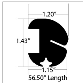
01456508 GLAZING, RUBBER, ENT DOOR, UPPER, STORM GLASS
