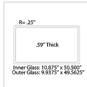
10032321 GLASS ASSY,STORM,O/O ENT DR,LWR,27.50,CV
