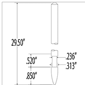
00046949 BOLT,SECURITY LOCK,OUTWARD OPENING DOOR
