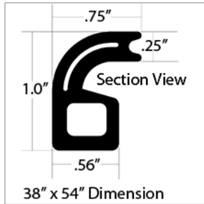
01360262 WEATHERSEAL,REAR EMERGENCY DOOR,RUBATEX
