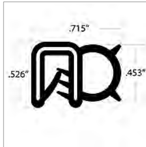
00124835 SEAL,REAR,EMERGENCY DOOR,AMBULANCE,D3FE
