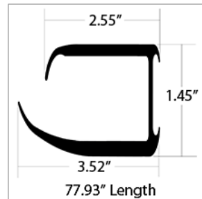
01383496 NOSING, RUBBER, ENT DOOR, JK, 36 AAF/RE
