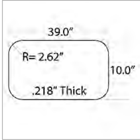
00347625 GLASS, DOOR, ENTRANCE, LOWER, TEMPERED
