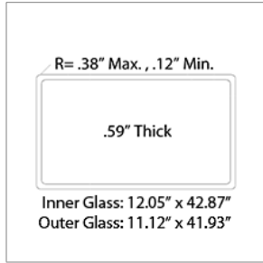
01602135 GLASS ASSY,STORM,ENT DR,LWR,24.75 TC AA
