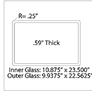
10032319 GLASS ASSY,STORM,O/O ENT DR,UPPER,CV
