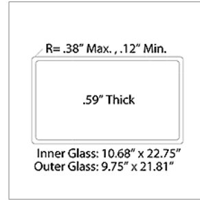
01602085 GLASS ASSY,STORM,ENT DR,UPPER,O/O CV
