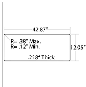
01472638 GLASS,DOOR,ENT,STL TUBE,LOWER,70PCT GRN AA
