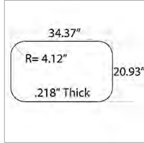
01110055 GLASS,RED,UPPER,CLEAR LAMINATED
