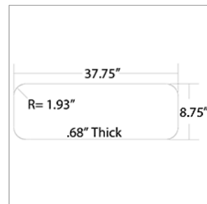
01565449 GLASS,DOOR,ENT,STORM,LOWER
