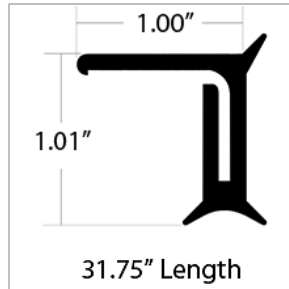
01651488 EXTRUSION, RUBBER, UPPER ENT DOOR SEAL, 31.75
