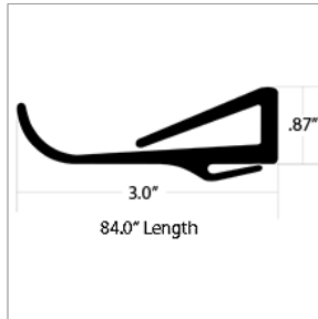
01373687 RUBBER,DOOR NOSING,FLUSH POWER JACKKNIFE DR
