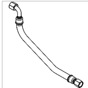
P-10D121-C-436 FUEL FILL LINE, 90 X STRAIGHT 10023470
