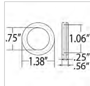
02003234 GROMMET, RUBBER, CHASSIS COWL WIRES, 3/4 IN ID
