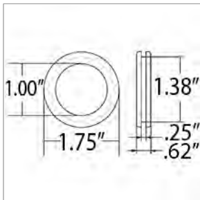
02003200 GROMMET, RUBBER, 1 IN ID
