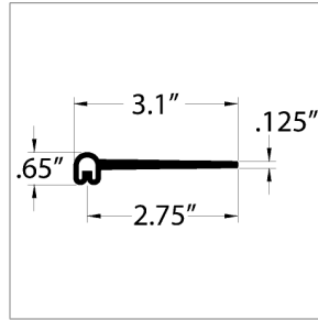
10044357 SEAL,CLOSEOUT,BATTERY BOX TO BODY
