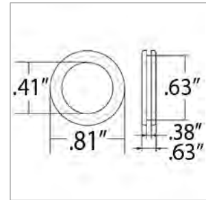
00066468 GROMMET, RUBBER, 13/32 ID, 3/8 GW, 5/8 GD
