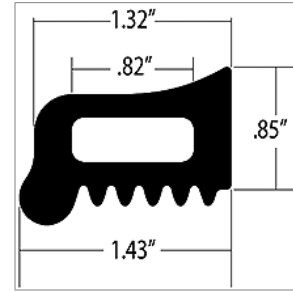
01489251 SEAL,ENGINE HOOD TCFC
