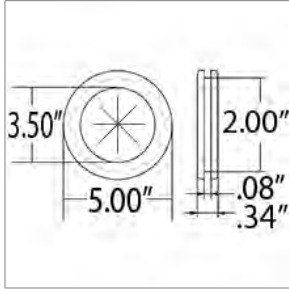
00058529 GROMMET, FIREWALL, 2 INCH, CLOSED
