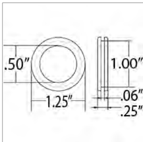
01508613 GROMMET, RUBBER, ATLANTIC INDIA #2426
