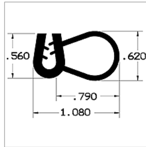
00116246 SEAL,RUBBER,RADIATOR BAFFLE M4RE
