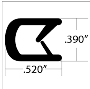
01489434 TRIM,VINYL,BLACK,DOUBLE LIP
