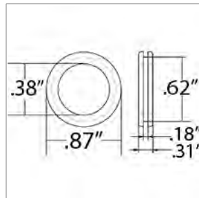
00890566 GROMMET, RUBBER, ATLANTIC INDIA, NO 2758
