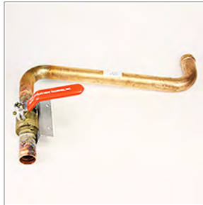
00063497 VALVE ASSY, HEATER, FRONT MAIN BBCV GMCV
