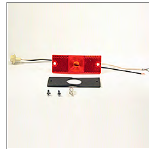
01941376 (Truck Lite® 18300R) LIGHT, MARKER, RECESSED, RED
