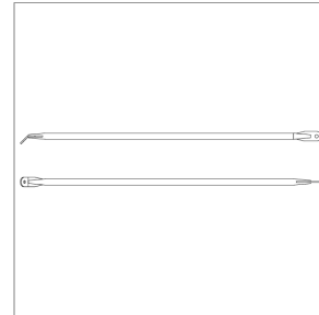
00072548 BRACE,MIRROR,30 ,LOWER,BLACK,ROSCO
