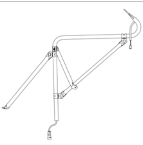
00083022 ARM ASSY,MIRROR,W/BRACES,LH,DRVR,STAINLESS STEEL
