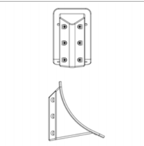
00024455 BASE,MOUNT,CROSSVIEW,(9018680)
