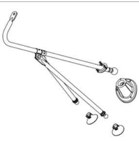
10030696 ARM,MIRROR,CROSSVIEW,W/BASE ASSEMBLY,LH, ROSCO
