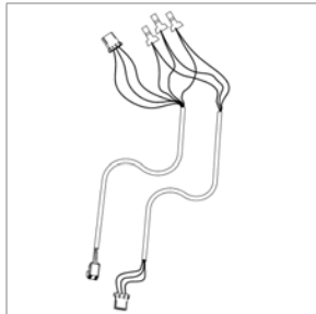
10001901 HARNESS,WIRING,MIRROR,PASSENGER,ROSCO
