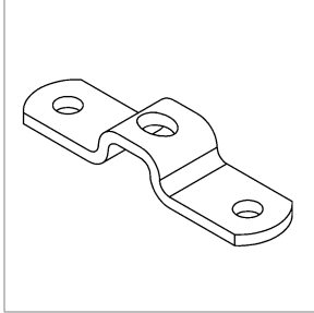
00068228 BRACKET,MTG,HIGH HAT,FLAT
