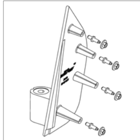
00073556 PLATE,MTG,MIRROR,PATCH MOUNT,DRV,FORD (2003 +)
