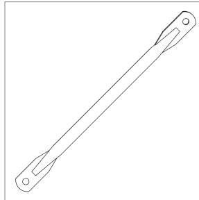
10010689 BRACE,MIRROR,BELL MTG,BLACK,15 TWIST,12 ,LH
