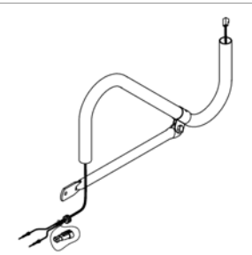
10021425 ARM ASSY,MIRROR,C-V,STAINLESS,HEATED,PASS SIDE,D3
