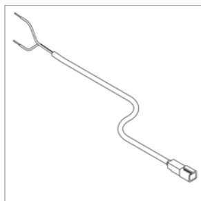
00043829 HARNESS,MIRROR,HTR,96 ,2 WIRE W/FEMALE CONNECTOR
