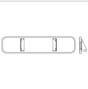
00046503 MIRROR,INTERIOR,6 X 30
