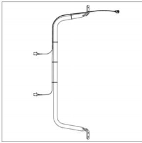
00127503 ARM ASSY,MIRROR,DRIVER,OPEN VIEW,ROSCO
