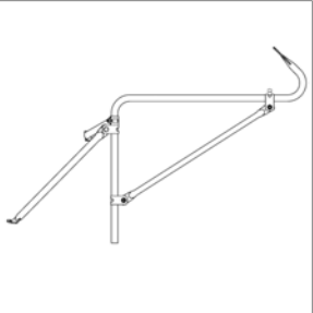
00086095 ARM ASSY,MIRROR,W/BRACES,RH SBCV IN33
