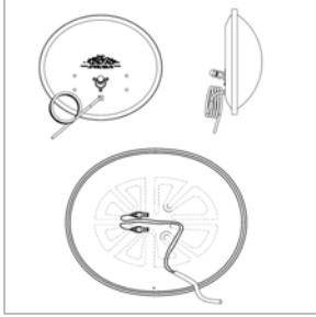
00024457 MIRROR HEAD,CROSSVIEW,HEATED (9018680)
