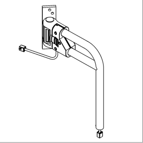
00042042 BASE,LH,FRTL,C/V
