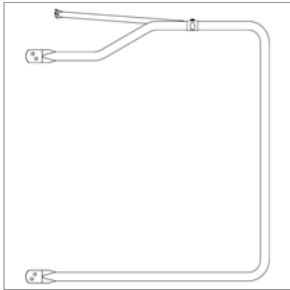
10022215 ARM ASSY,MIRROR,SS,PASS S,OPEN VIEW ES,D3
