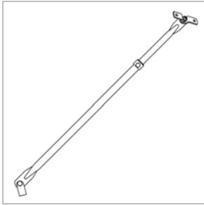
00115886 KIT,BRACE,MIRROR,TELESCOPING,18-24 ,BLACK
