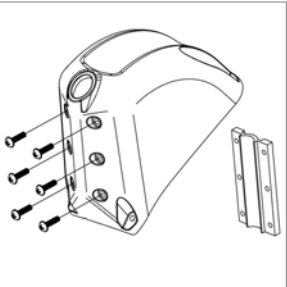
00113315 BASE,MTG,MIRROR,C/V,DRIVER
