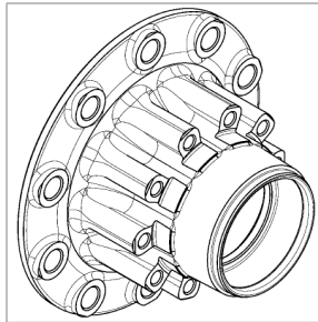
10041184 HUB & CUP ASSY,STEER,HYDRAULIC BRK,FF SPINDLE
