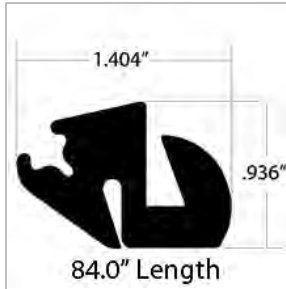
00962746 GLAZING,RUBBER,84
