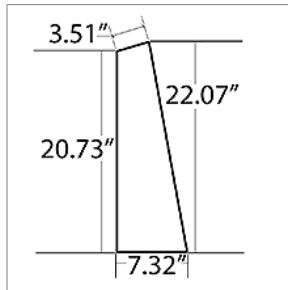
00218172 GLASS,WINDSHIELD,CORNER,CLEAR,SAFETY PLATE
