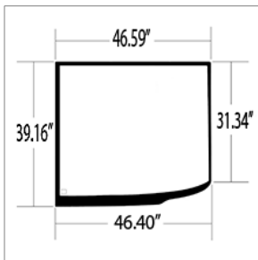
10029996 GLASS,WINDSHIELD,CURVED,RH,SHADED,T3
