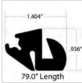
00034771 GLAZING,RUBBER,RED,LOWER,79.00 SRWAFFD/GM
