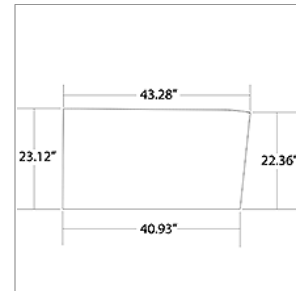
00357368 GLASS,W-S,CNTR,TINTED
