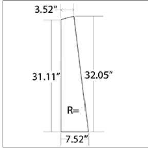
01532399 GLASS,W-S,CORNER,4FF,,265,AUTO TINT,20.09BB
