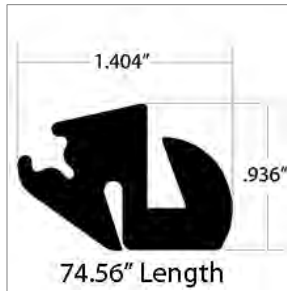
01114321 GLAZING,RUBBER,74.5625
