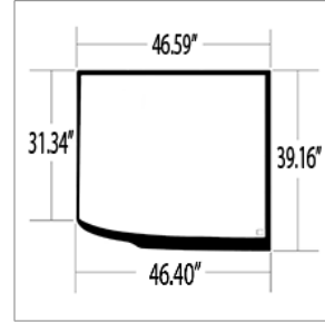
10029998 GLASS,WINDSHIELD,CURVED,LH,SHADED,T3
