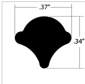
00269373 FILLERSTRIP,GLAZING RUBBER
