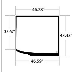
00125620 GLASS,WINDSHIELD,CURVED,LH,SHADED D3
