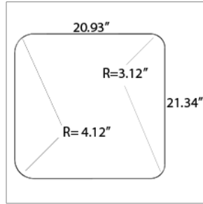
01110162 GLASS,REAR VISION,CLEAR,LAMINATED
