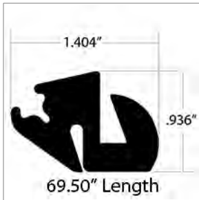
00949107 GLAZING,RUBBER,69 1/2 MBCC
