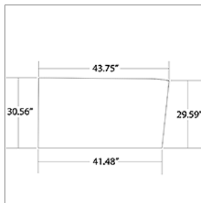
01327014 GLSSS,W/S,CNTR,CLEAR,4FF TCFC
