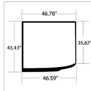
00125619 GLASS,WINDSHIELD,CURVED,RH,SHADED D3
