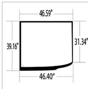
10029995 GLASS,WINDSHIELD,CURVED,RH,TINTED,T3
