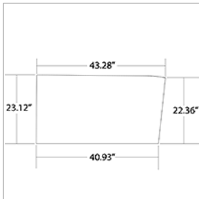
00357293 GLASS,WINDSHIELD,CNTR,CLR,SFTY PLT,FLAT,FR
