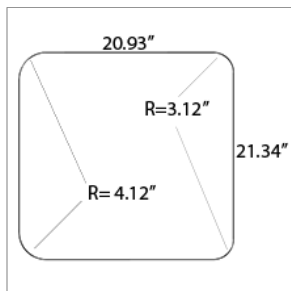
01110154 GLASS,REAR VISION,TEMPERED
