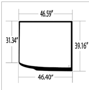
10029997 GLASS,WINDSHIELD,CURVED,LH,TINTED,T3
