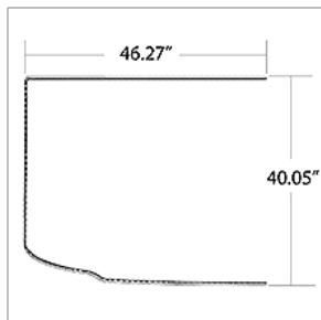
10030000 TRIM,WINDSHIELD,OUTER PERIMETER,LH,T3
