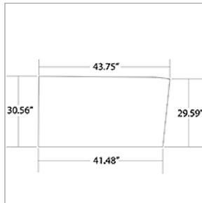
00357301 GLASS,W/S,TINTED,4FF,CENTER
