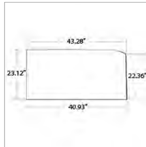
00357376 GLASS,W-S,CNTR,SHADED,SAFETY PLATE
