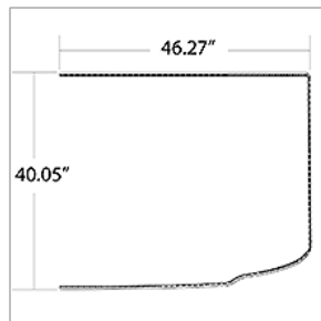
10029999 TRIM,WINDSHIELD,OUTER PERIMETER,RH,T3
