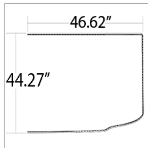
10005263 TRIM,SEAL,WINDSHIELD,OUTER,LH,D3
