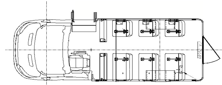
Seating for 9 passengers plus the driver, including center aisle for passenger ease of loading
